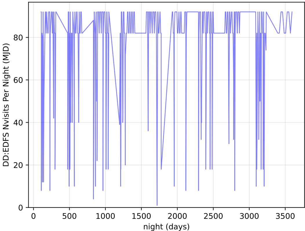
weather_cloudso1v3.4_10yrs all bands: DD:EDFS Nvisits Per Night
