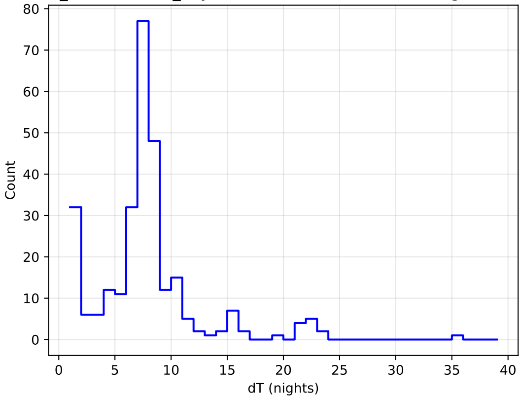
weather_cloudso1v3.4_10yrs all bands: DD:EDFS Delta Nights Histogram
