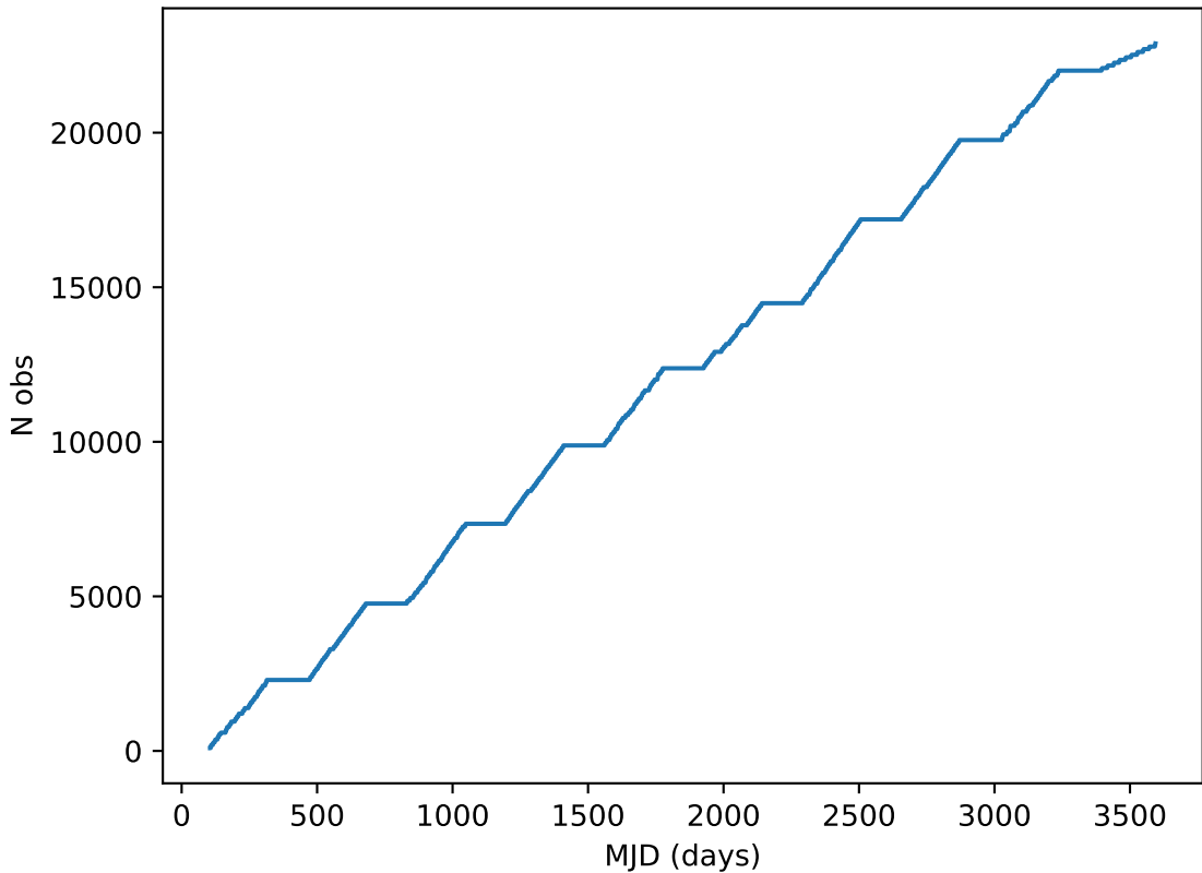
weather_cloudso1v3.4_10yrs all bands: DD:EDFS Cumulative NVisits
