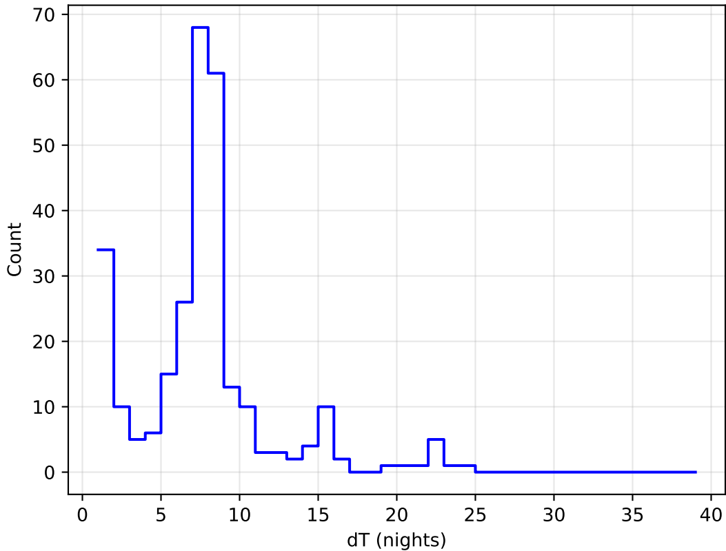
weather_cloudso1v3.4_10yrs all bands: DD:ECDFS Delta Nights Histogram
