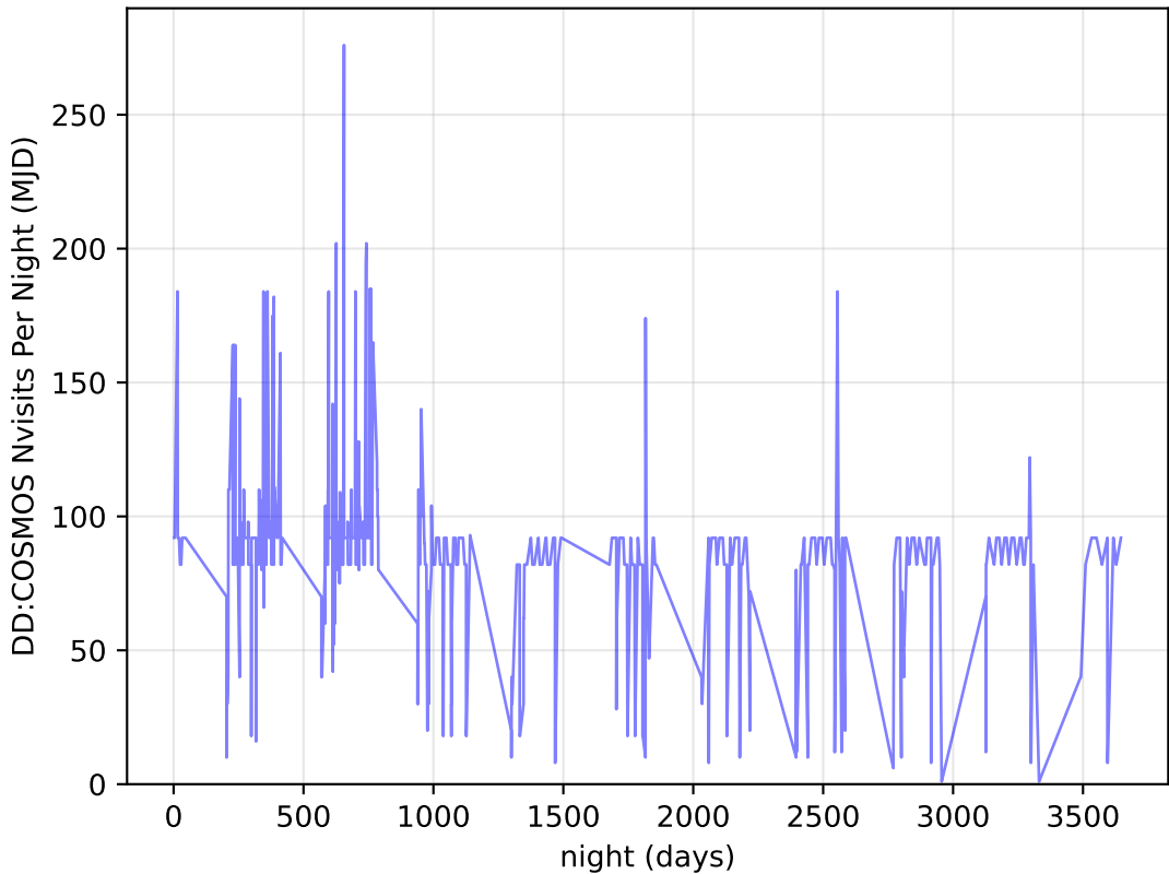
weather_cloudso1v3.4_10yrs all bands: DD: COSMOS Nvisits Per Night
