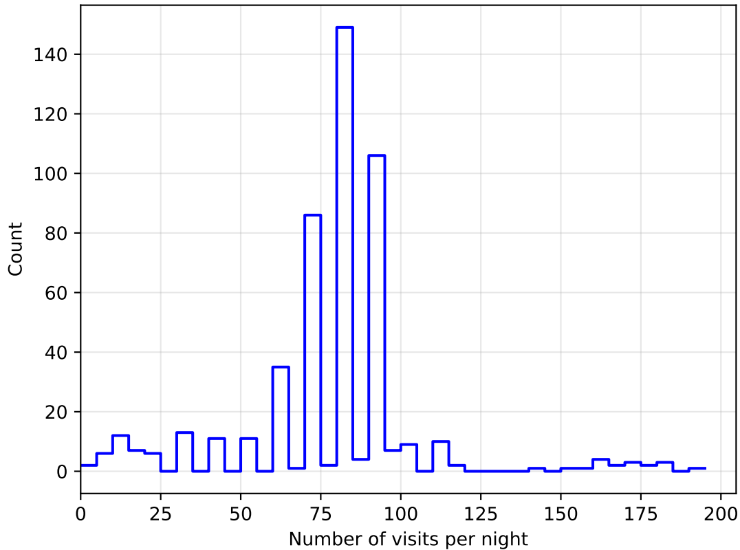
weather_cloudso1v3.4_10yrs all bands: DD: COSMOS NVisitsPerNight
