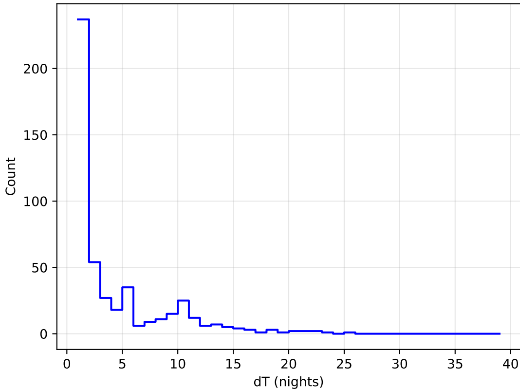
weather_cloudso1v3.4_10yrs all bands: DD: COSMOS Delta Nights Histogram
