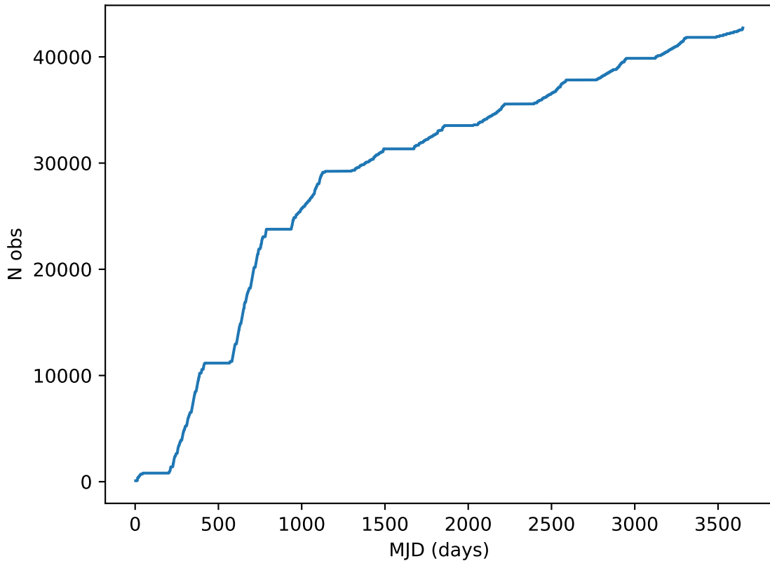
weather_cloudso1v3.4_10yrs all bands: DD:COSMOS Cumulative NVisits
