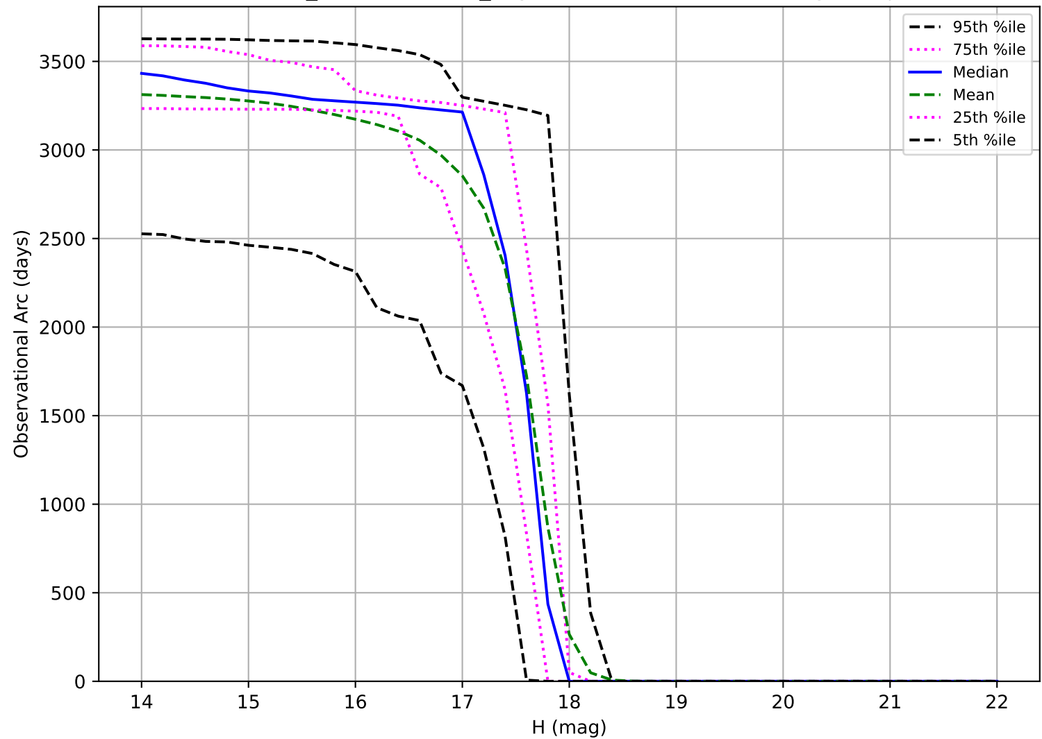
weather_cloudso18v3.4_10yrs: Observational Arc Length Trojan
