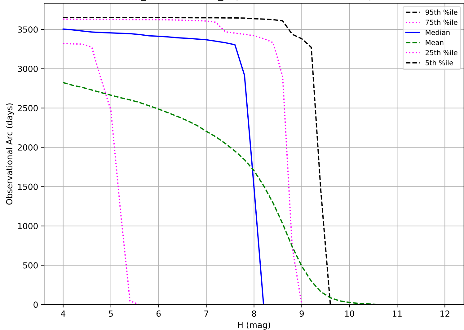
weather_cloudso18v3.4_10yrs: Observational Arc Length TNO
