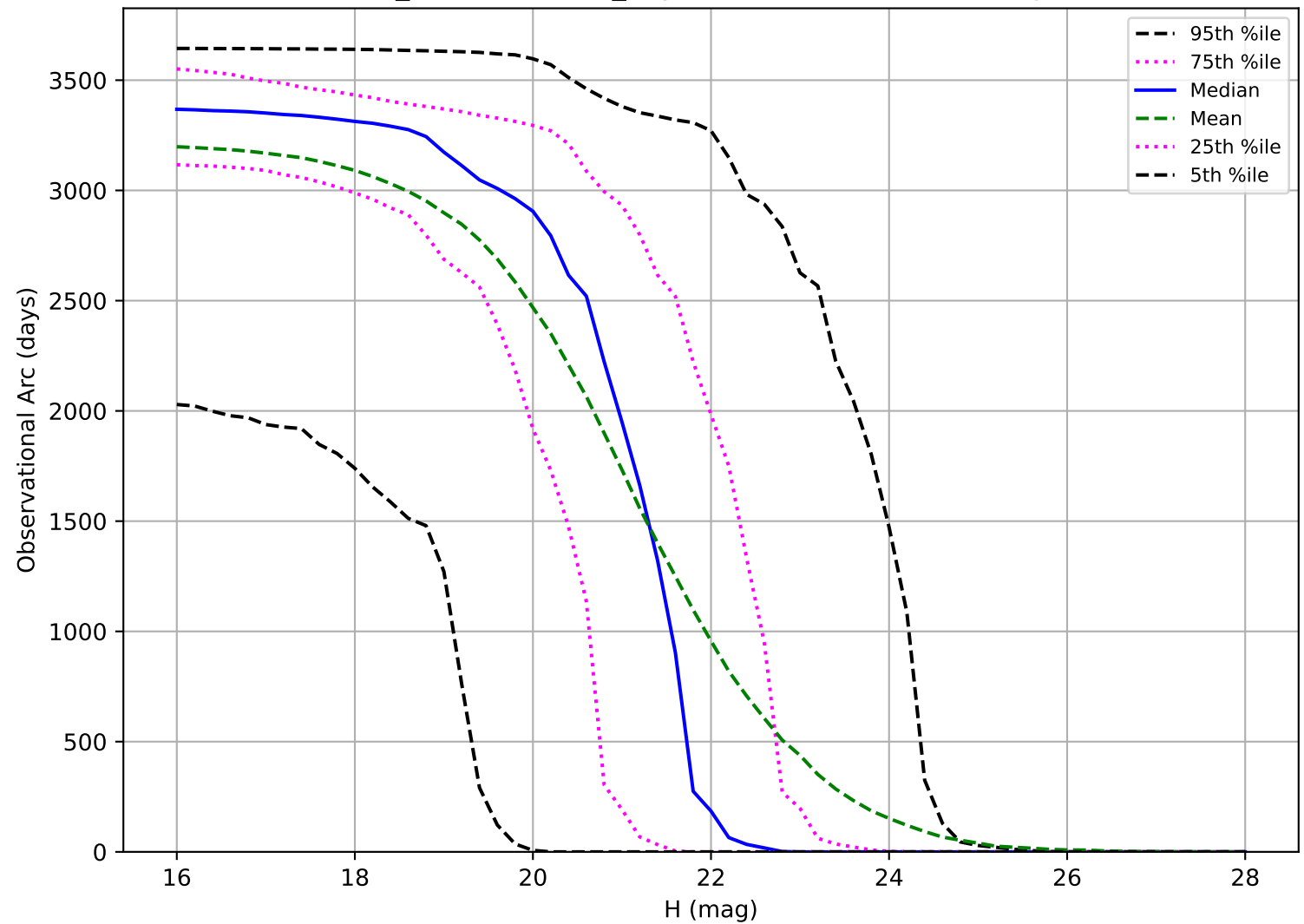
weather_cloudso18v3.4_10yrs: Observational Arc Length PHA
