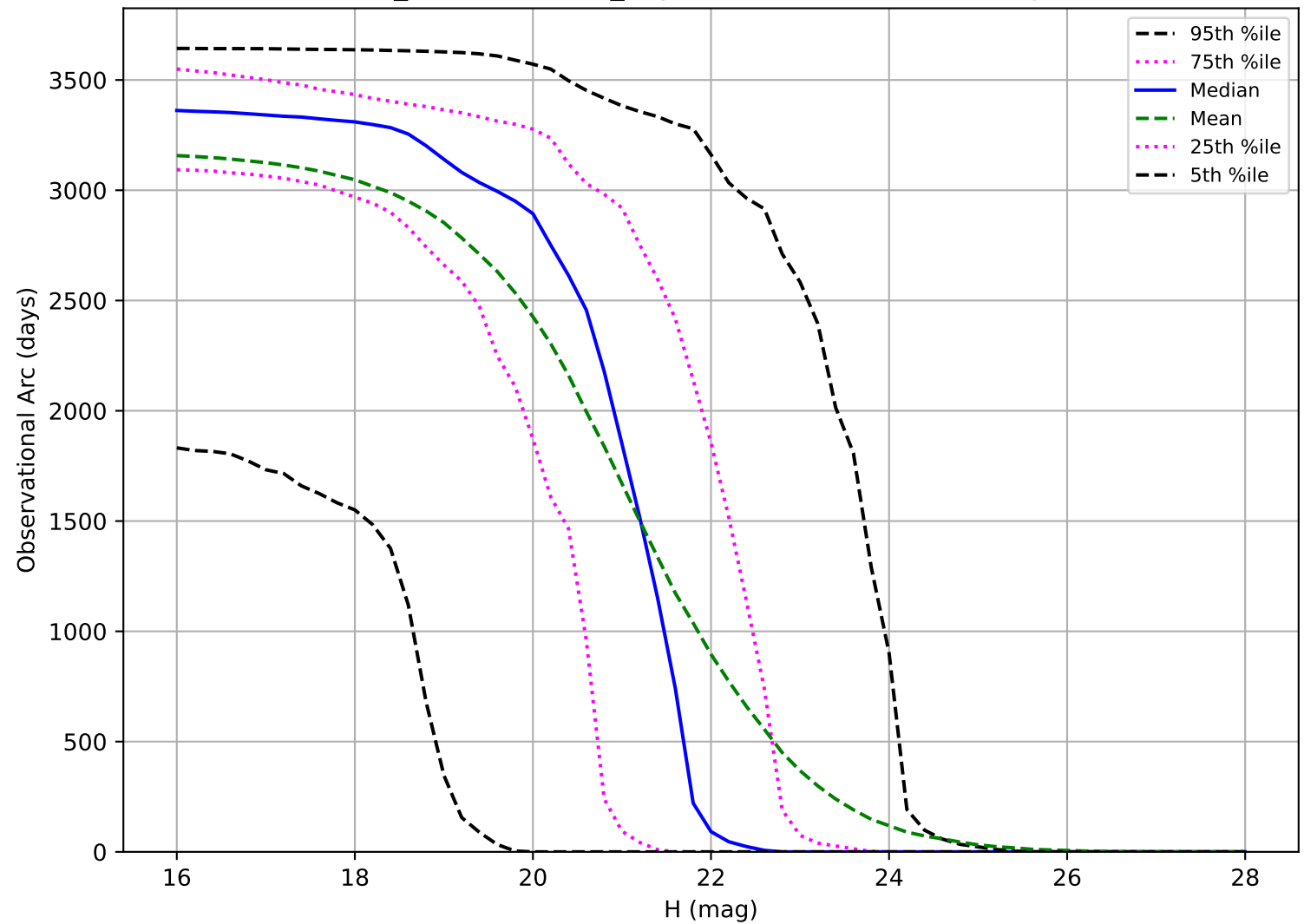
weather_cloudso18v3.4_10yrs: Observational Arc Length NEO
