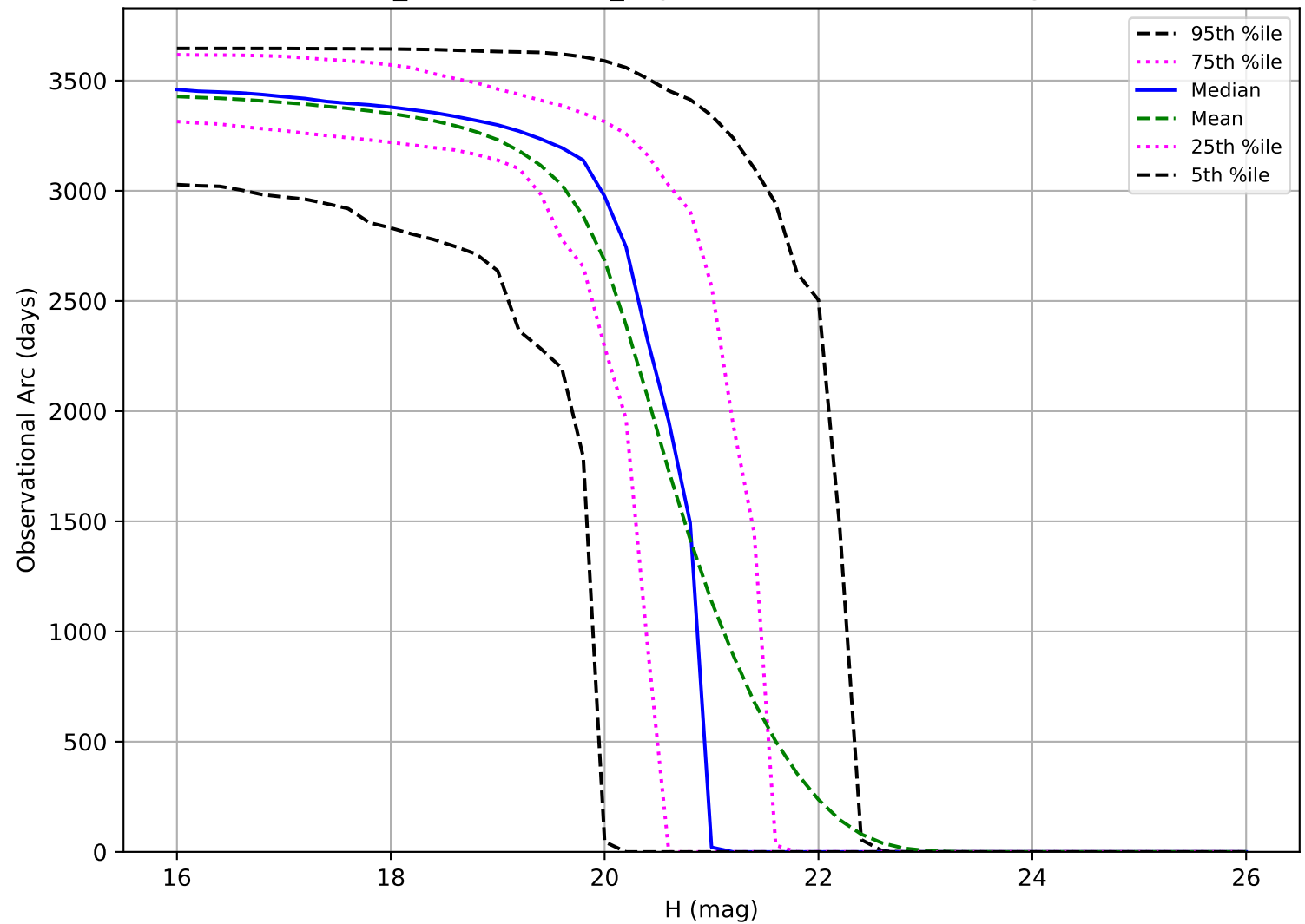
weather_cloudso18v3.4_10yrs: Observational Arc Length MBA
