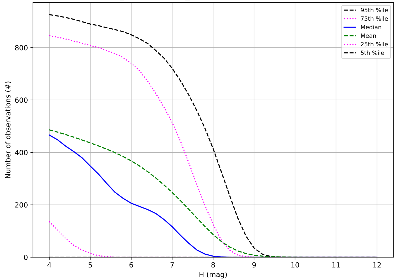
weather_cloudso18v3.4_10yrs: Number of observations TNO
