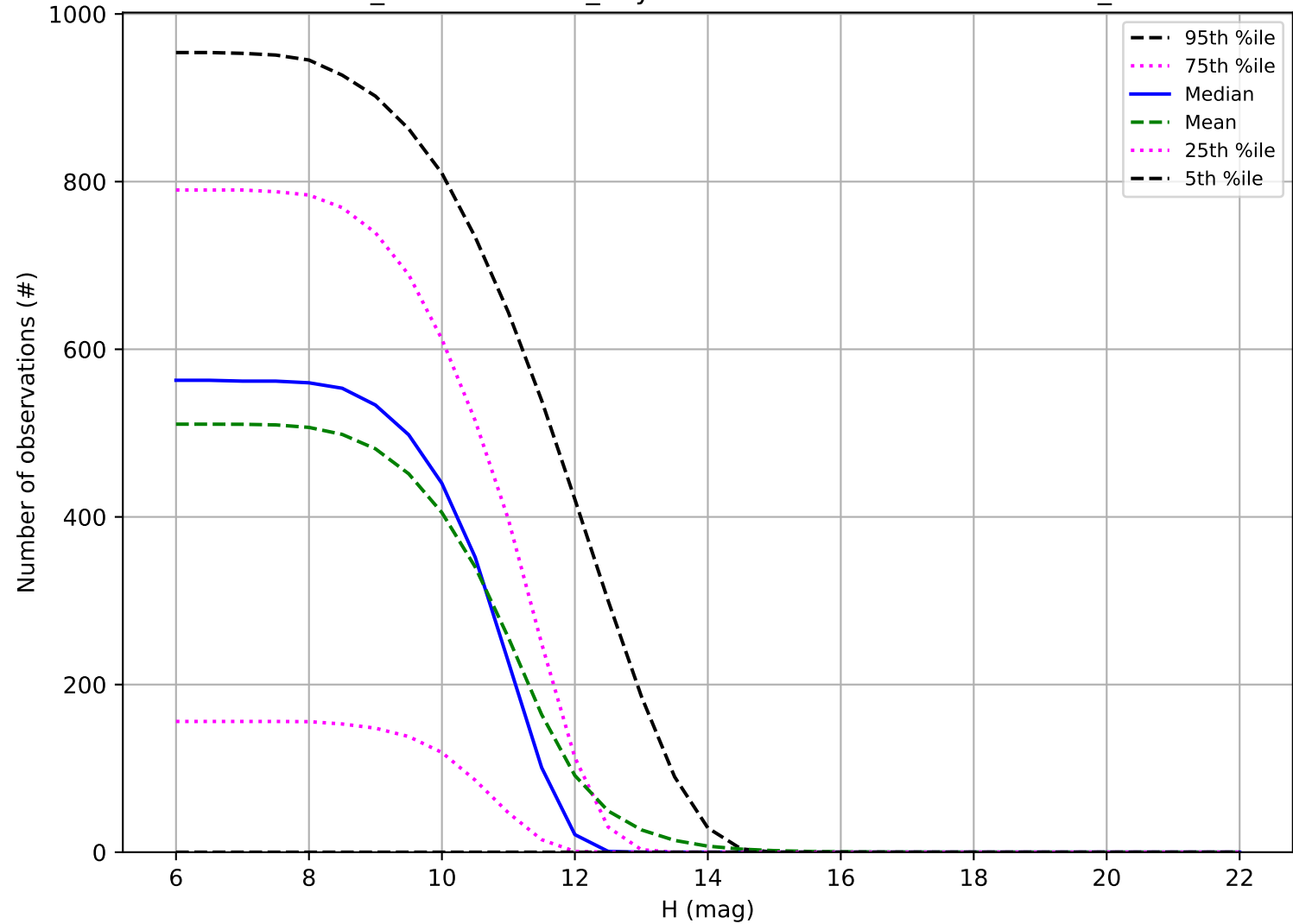
weather_cloudso18v3.4_10yrs: Number of observations OCC_r20
