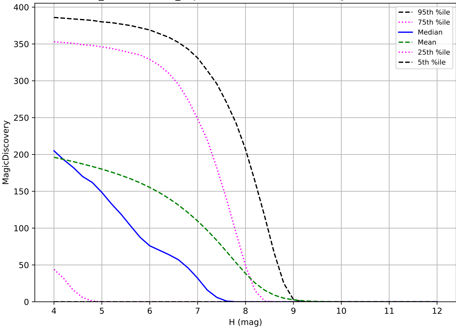
weather_cloudso18v3.4_10yrs: TNO 6 detections in 60 nights detection loss
