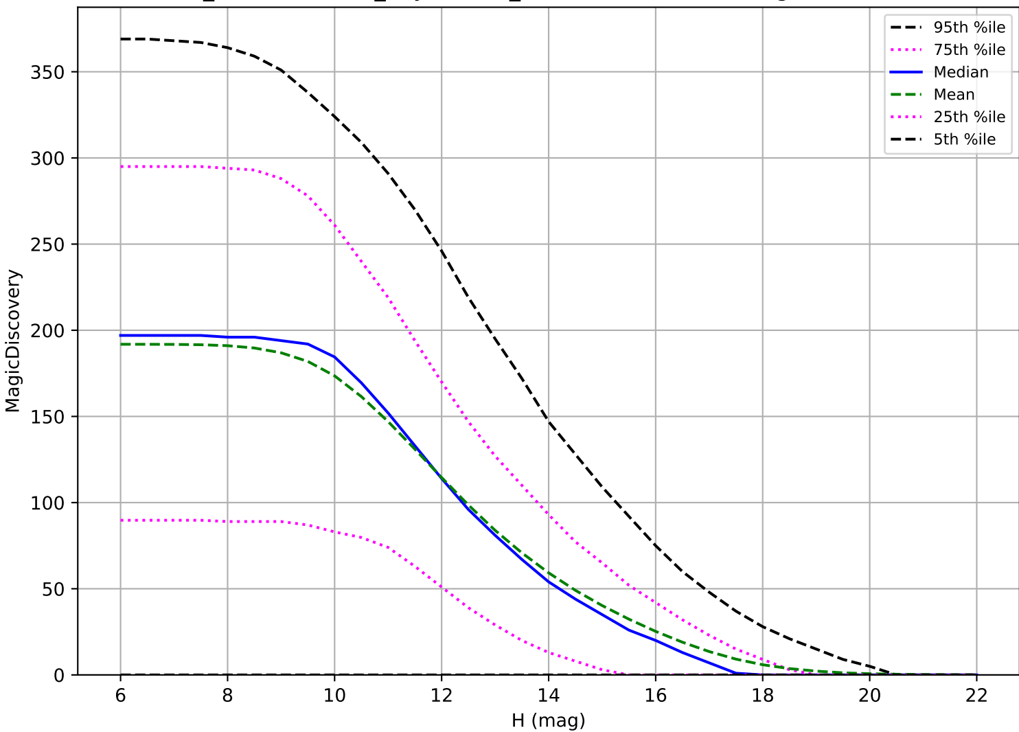
weather_cloudso18v3.4_10yrs: OCC_r5 6 detections in 60 nights detection loss
