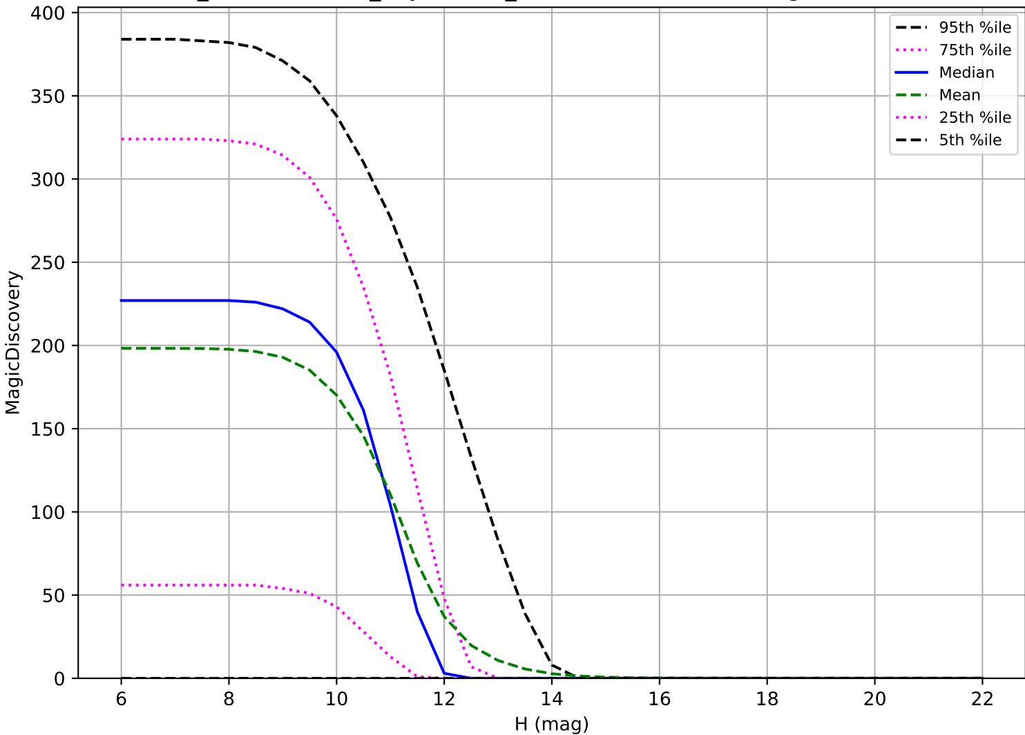
weather_cloudso18v3.4_10yrs: OCC_r20 6 detections in 60 nights detection loss
