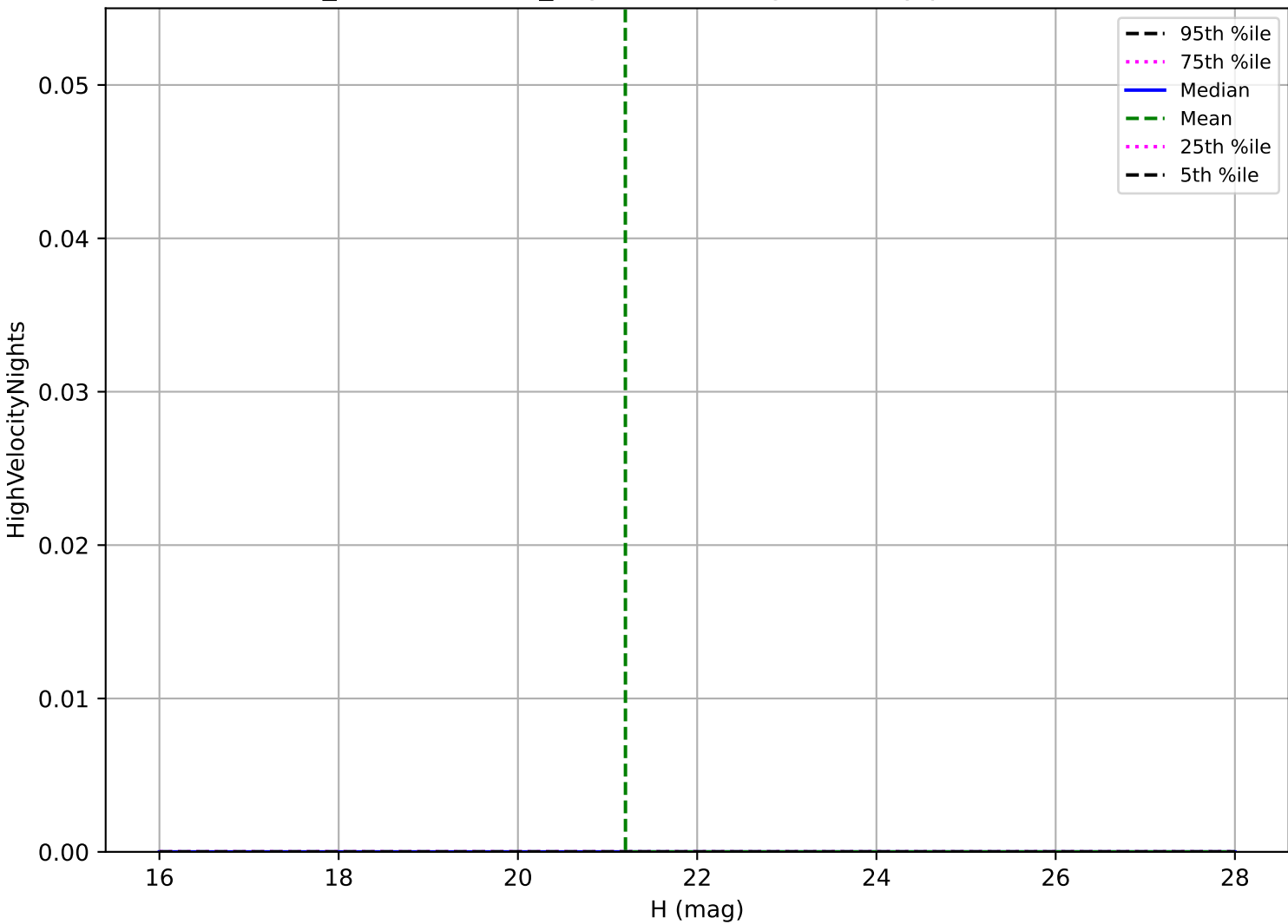
weather_cloudso18v3.4_10yrs: Vatira High velocity pair detection loss
