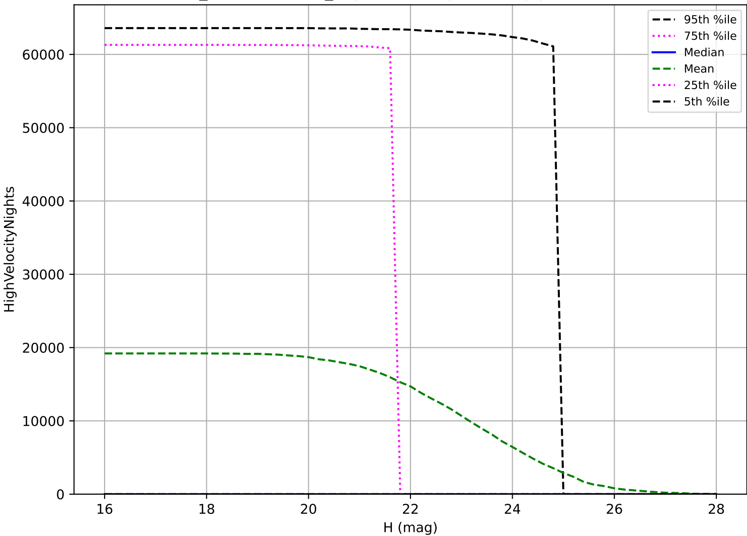
weather_cloudso18v3.4_10yrs: NEO High velocity pair detection loss
