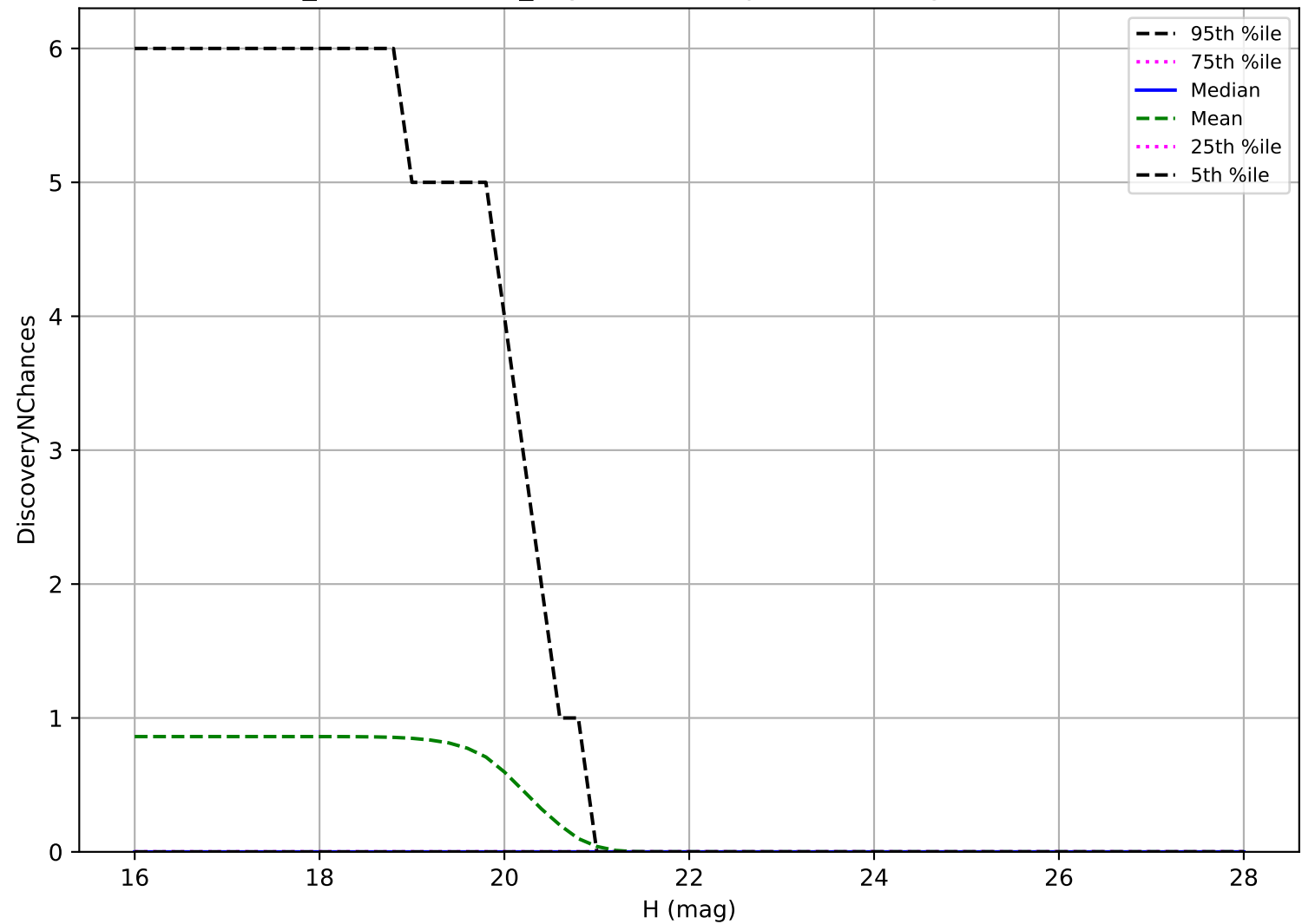
weather_cloudso18v3.4_10yrs: Vatira 3 pairs in 15 nights detection loss
