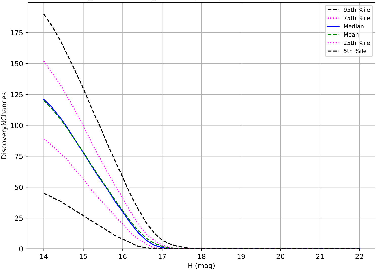
weather_cloudso18v3.4_10yrs: Trojan 3 pairs in 15 nights detection loss
