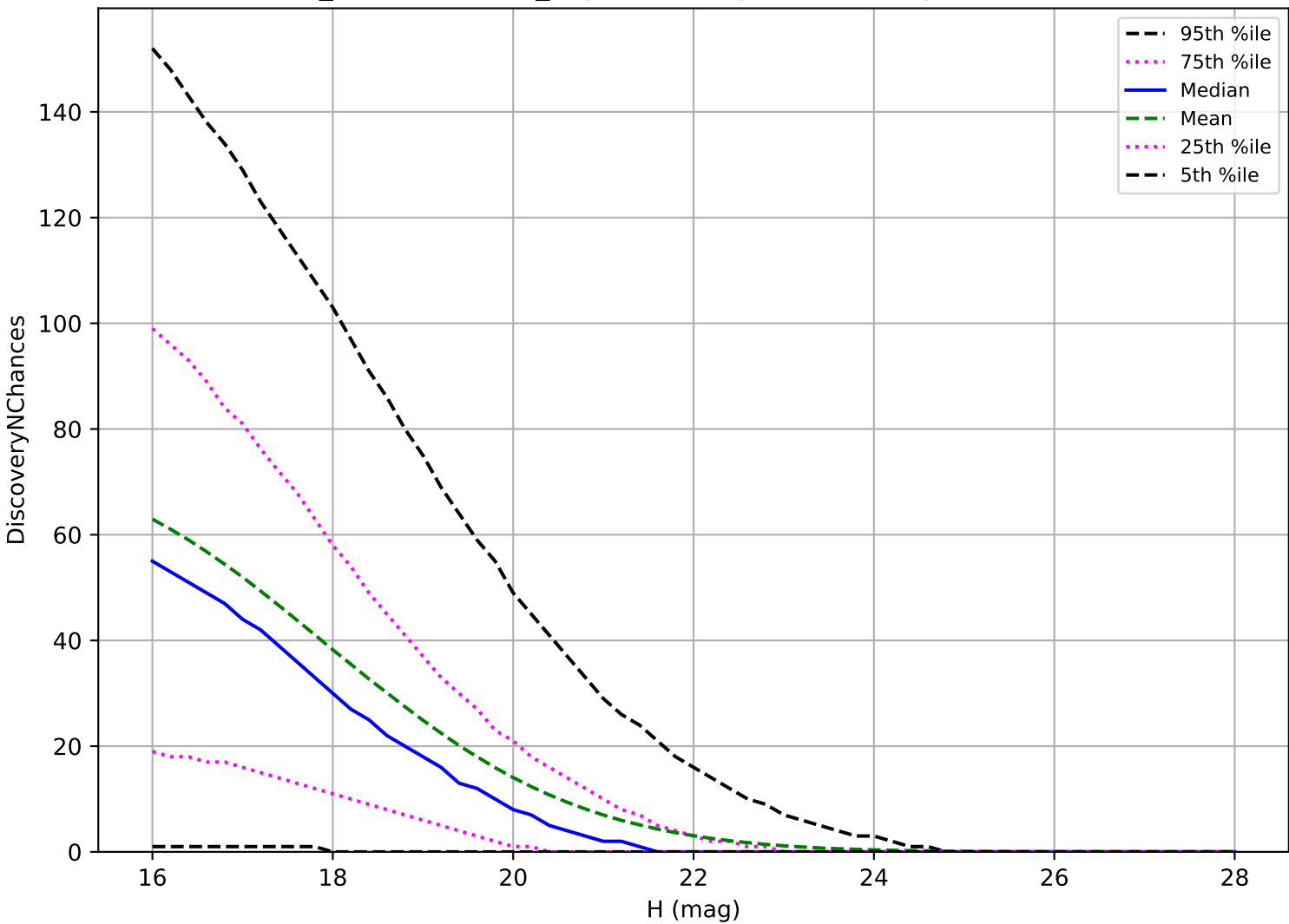
weather_cloudso18v3.4_10yrs: PHA 3 pairs in 15 nights detection loss
