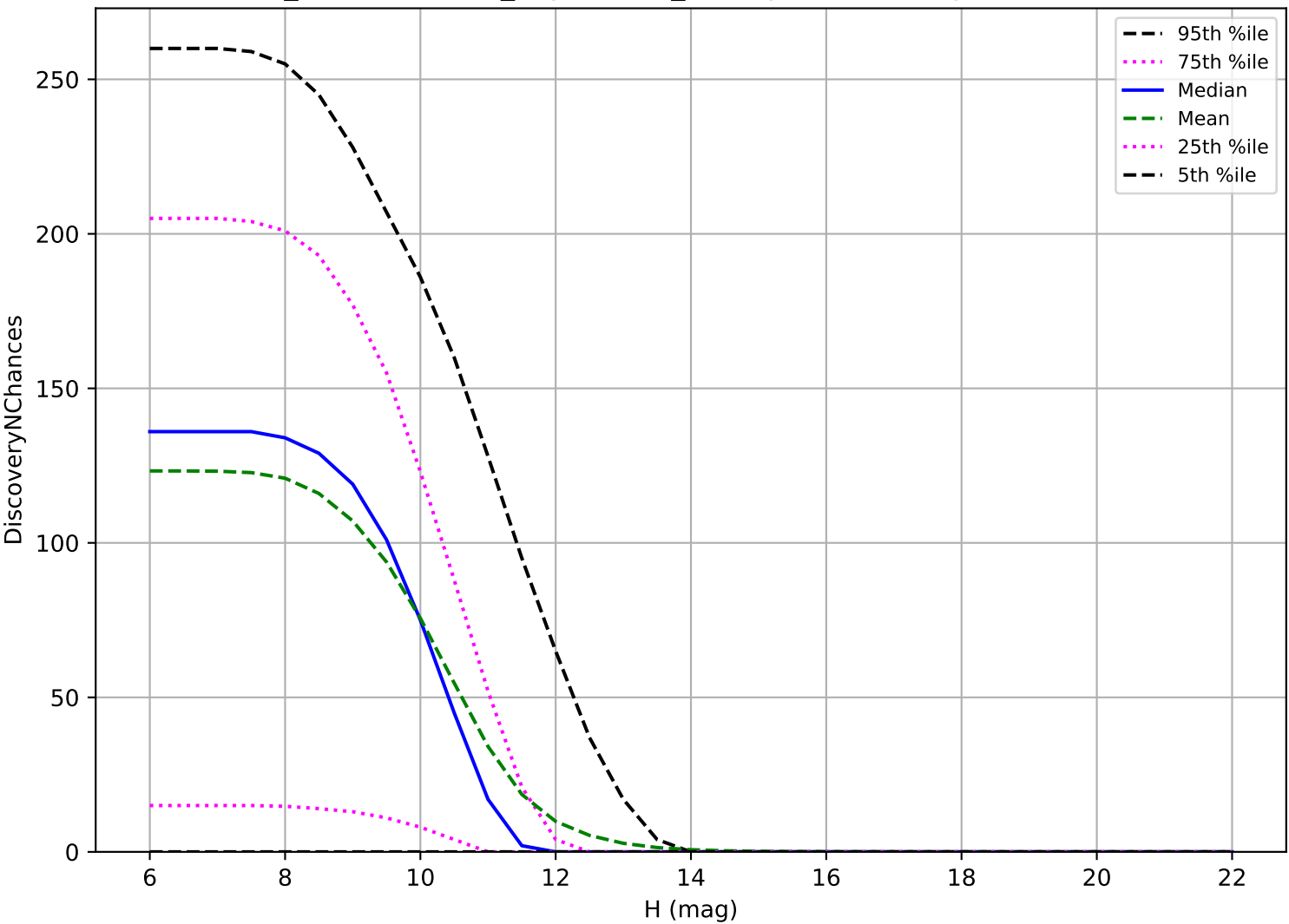
weather_cloudso18v3.4_10yrs: OCC_r20 3 pairs in 15 nights detection loss
