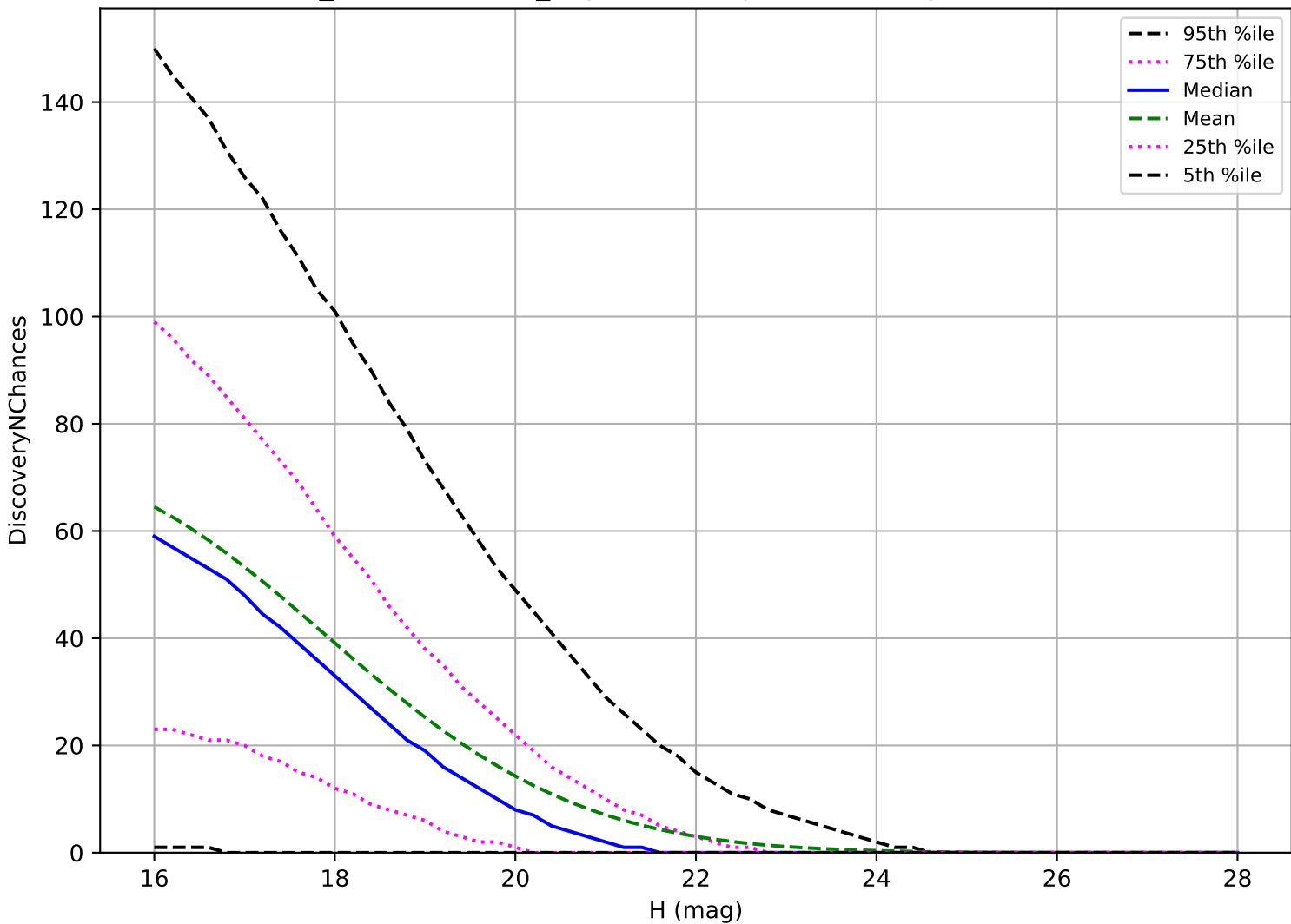
weather_cloudso18v3.4_10yrs: NEO 3 pairs in 15 nights detection loss
