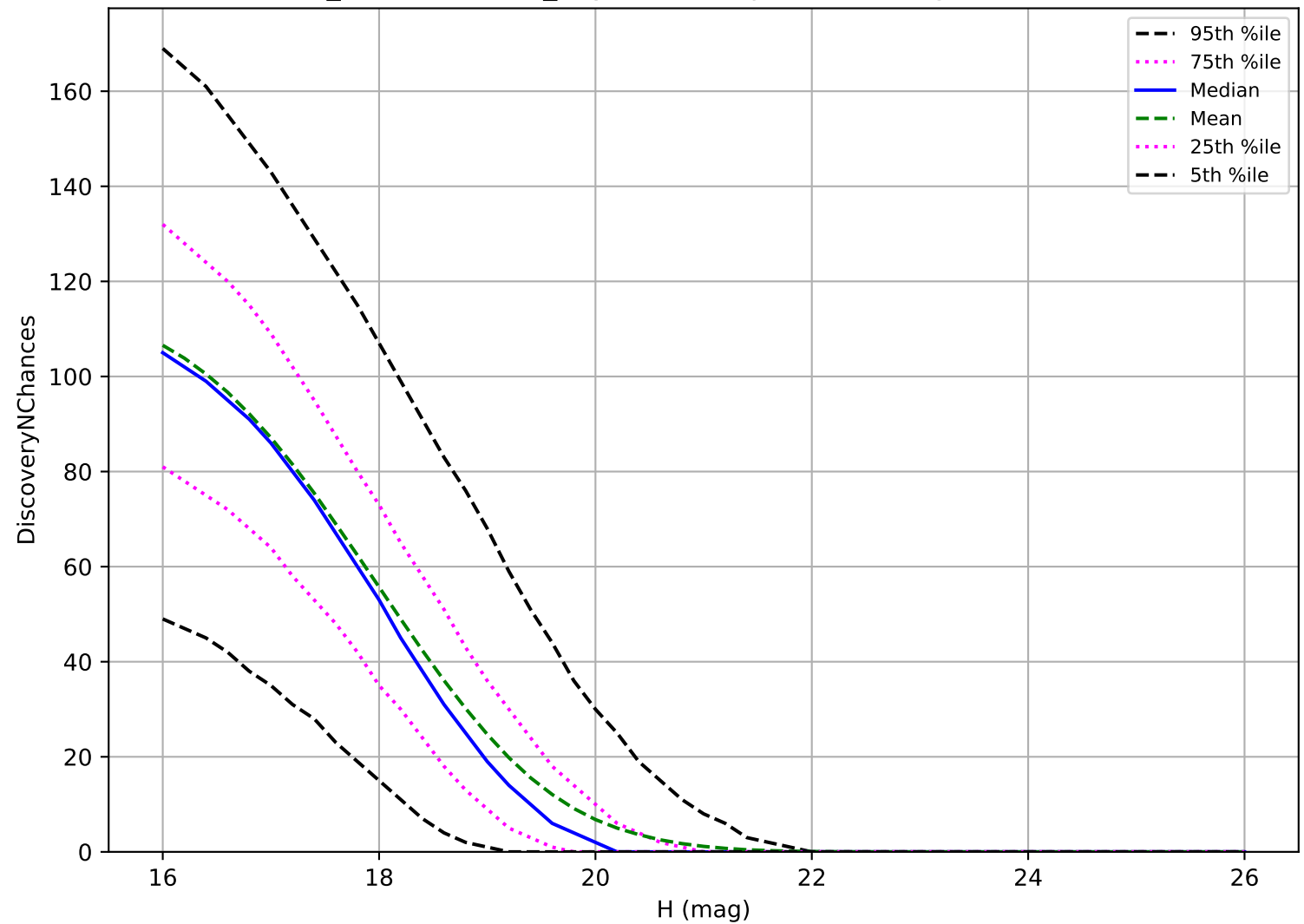
weather_cloudso18v3.4_10yrs: MBA 3 pairs in 15 nights detection loss
