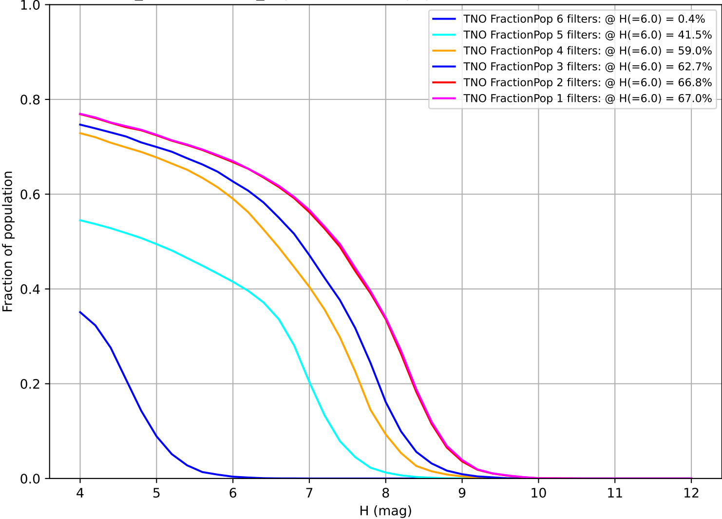
weather_cloudso18v3.4_10yrs: Fraction of population with colors in X filters TNO
