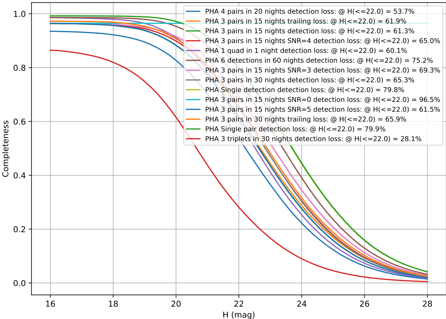
weather_cloudso18v3.4_10yrs: CumulativeCompleteness
