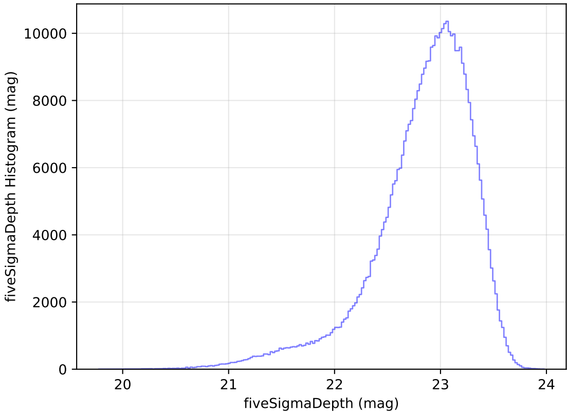
weather_cloudso18v3.4_10yrs z: fiveSigmaDepth Histogram
