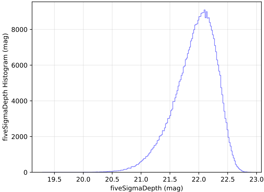
weather_cloudso18v3.4_10yrs y: fiveSigmaDepth Histogram
