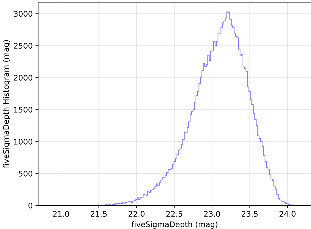
weather_cloudso18v3.4_10yrs u: fiveSigmaDepth Histogram
