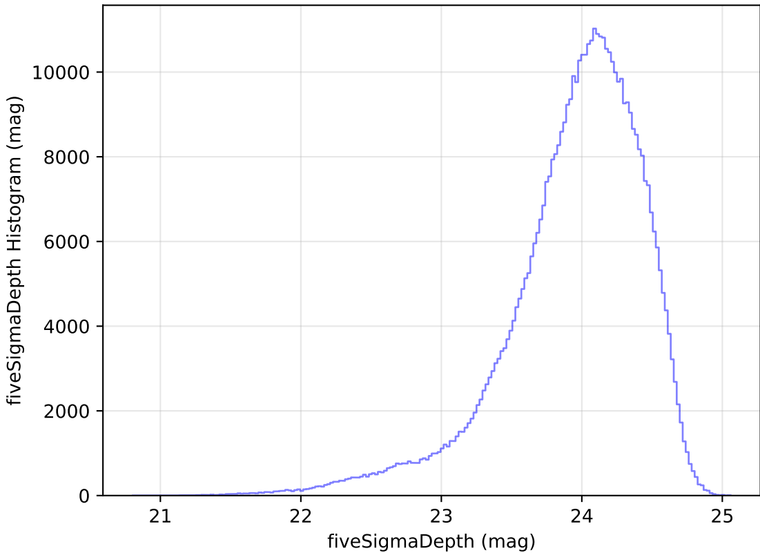
weather_cloudso18v3.4_10yrs r: fiveSigmaDepth Histogram
