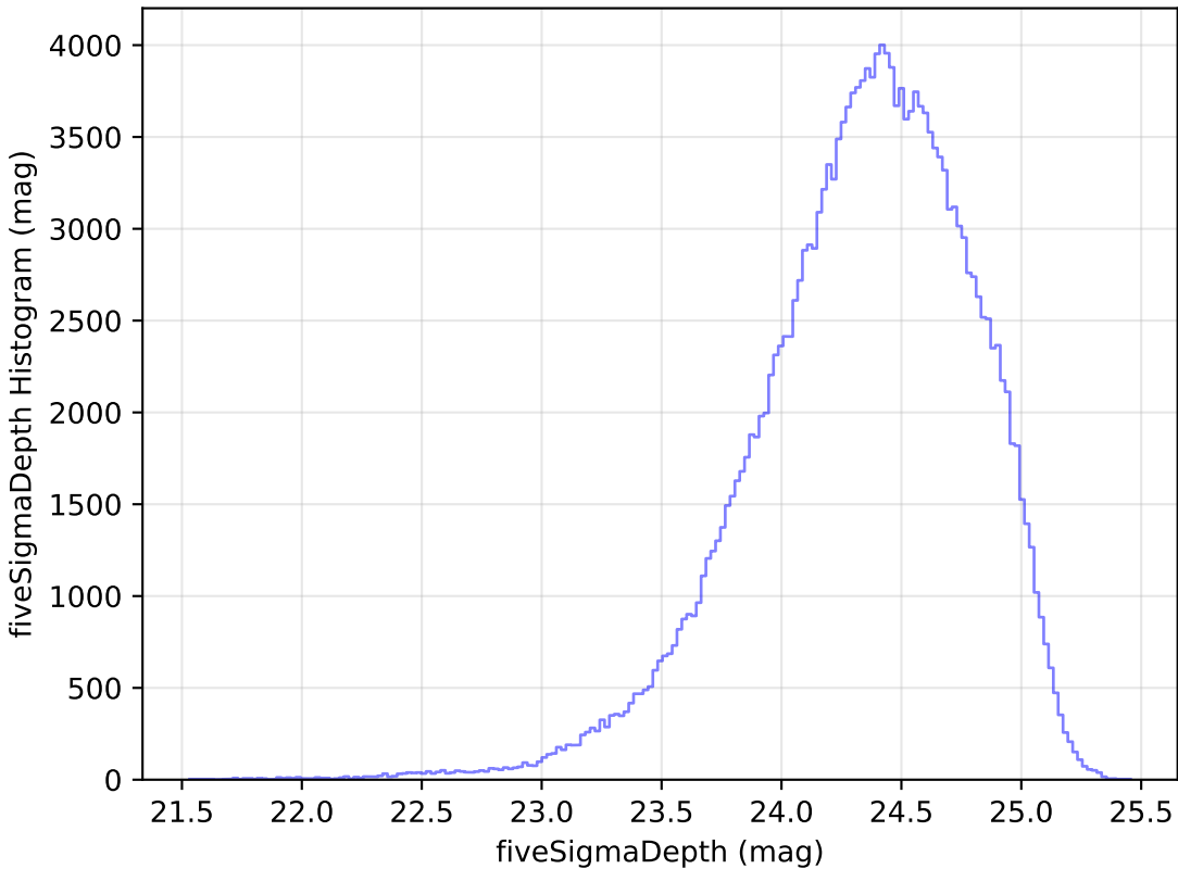
weather_cloudso18v3.4_10yrs g: fiveSigmaDepth Histogram
