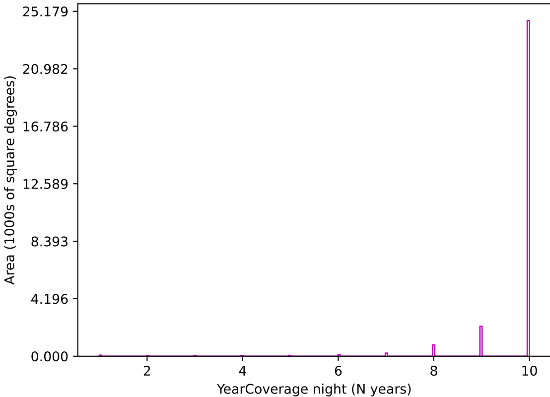
weather_cloudso18v3.4_10yrs z band: YearCoverage night
