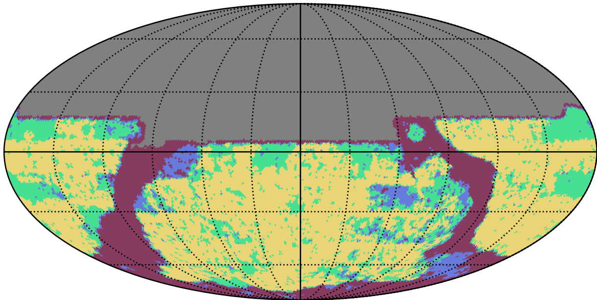
weather_cloudso18v3.4_10yrs u band: YearCoverage night
