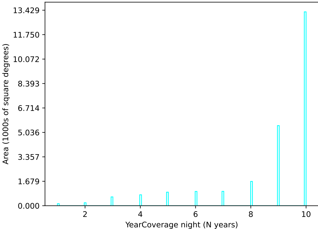
weather_cloudso18v3.4_10yrs u band: YearCoverage night
