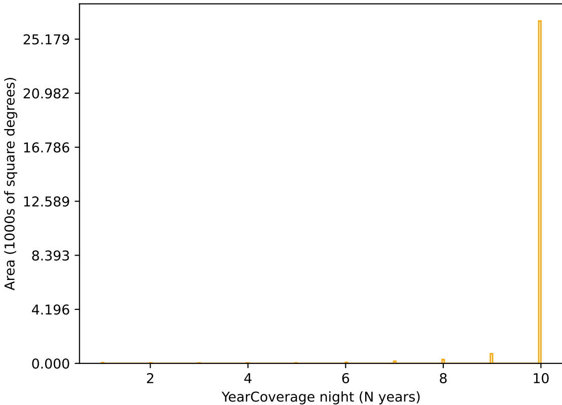
weather_cloudso18v3.4_10yrs r band: YearCoverage night
