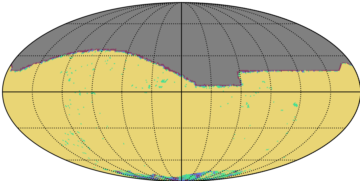
weather_cloudso18v3.4_10yrs i band: YearCoverage night
