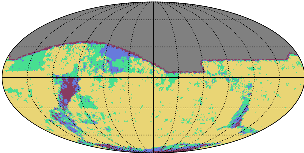
weather_cloudso18v3.4_10yrs g band: YearCoverage night
