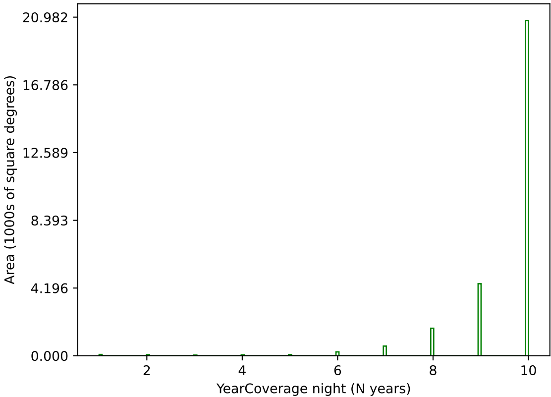
weather_cloudso18v3.4_10yrs g band: YearCoverage night
