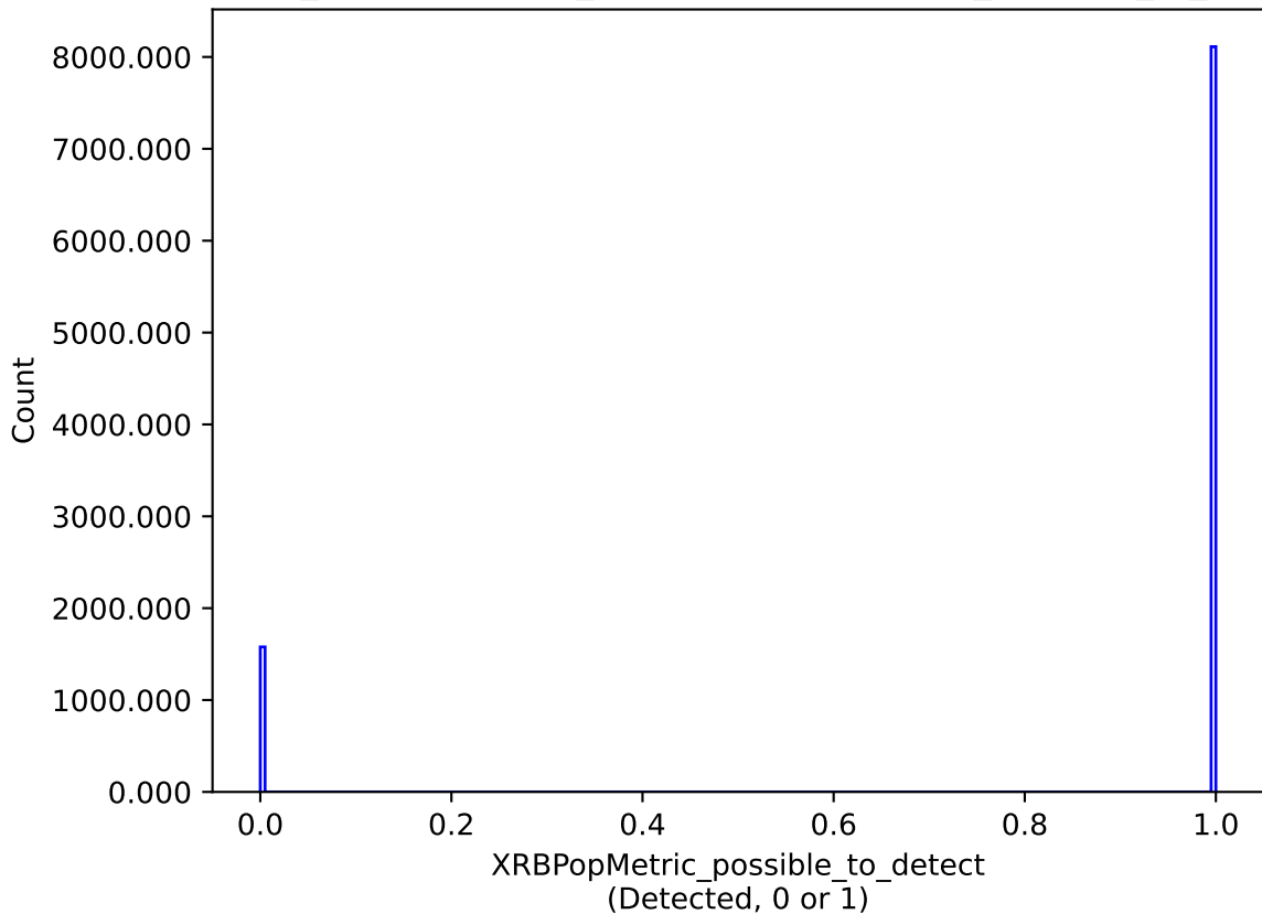
weather_cloudso18v3.4_10yrs : XRBPoMetric_possible_to_detect
