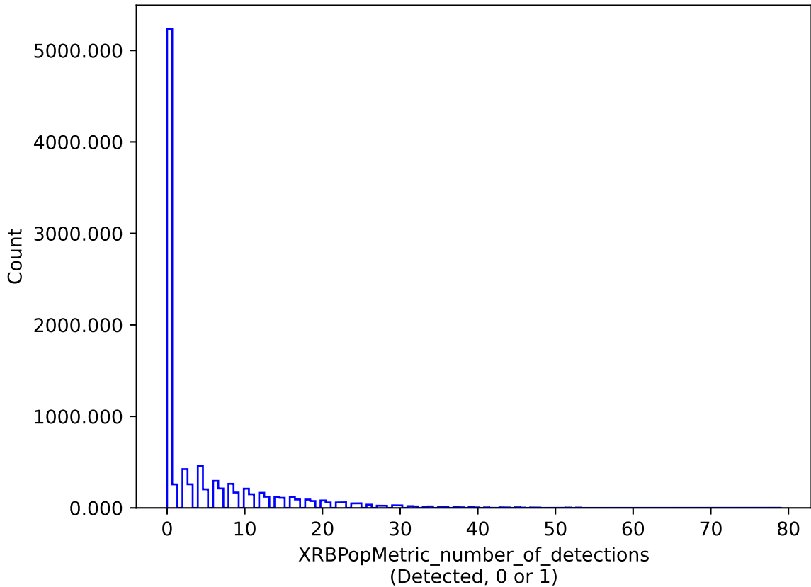
weather_cloudso18v3.4_10yrs : XRBPoMetric_number_of_detections
