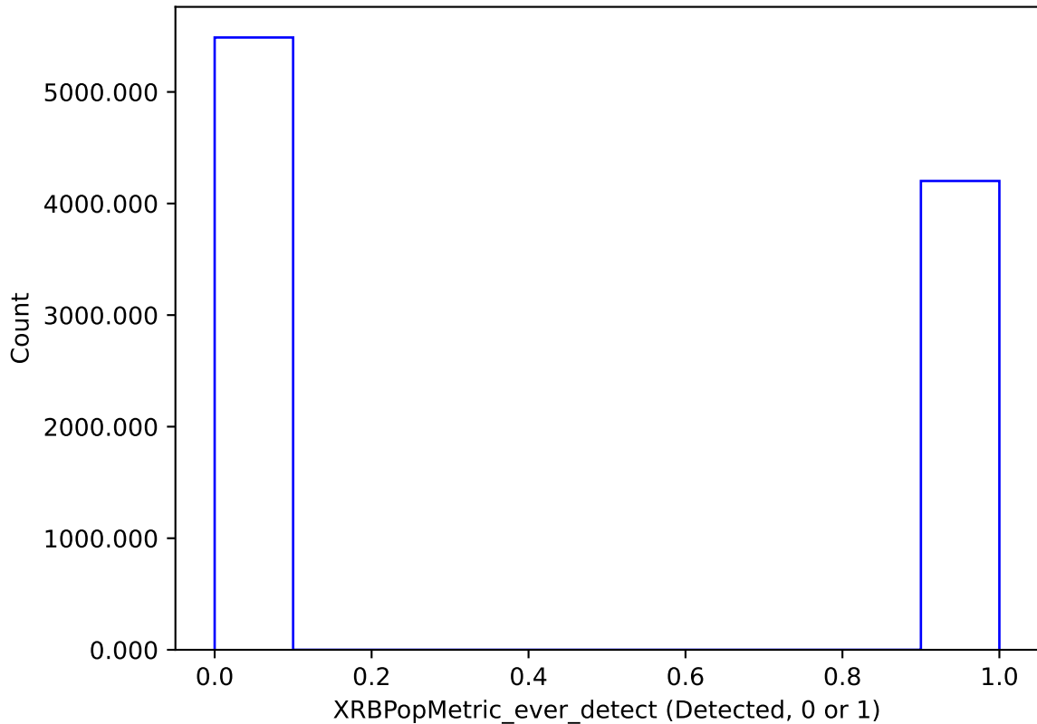
weather_cloudso18v3.4_10yrs : XRBPoMetric_ever_detect
