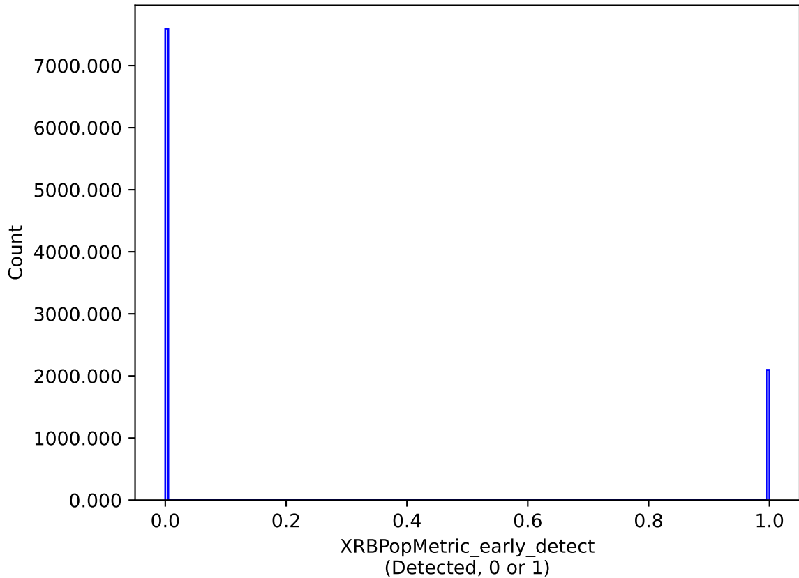
weather_cloudso18v3.4_10yrs : XRBPoMetric_early_detect
