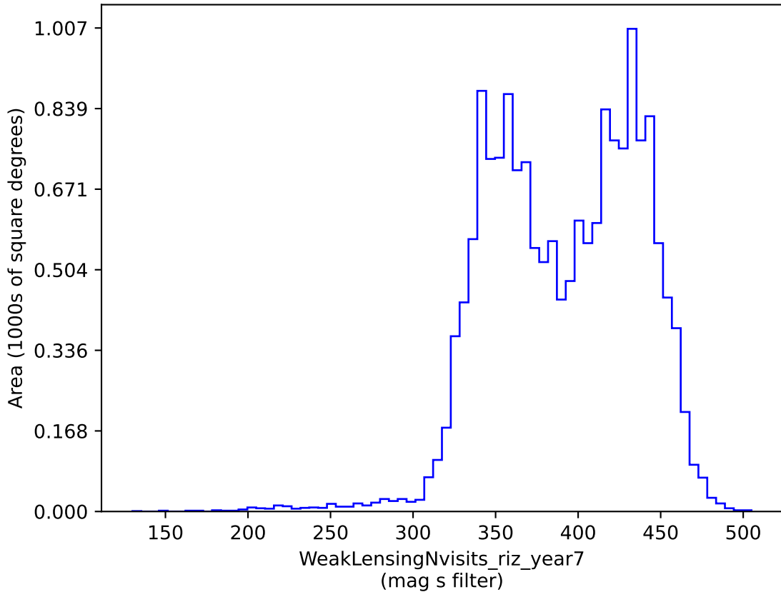
weather_cloudso18v3.4_10yrs gri band non-DD: WeakLensingNvisits_riz_year7
