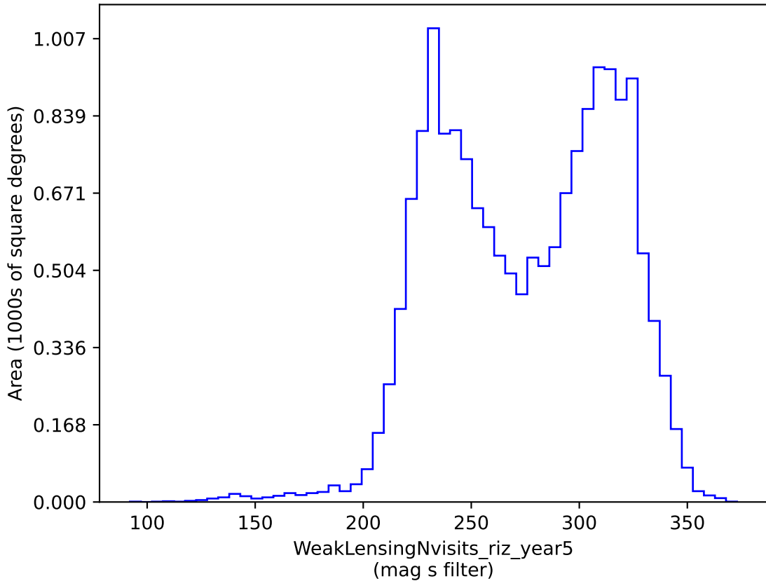
weather_cloudso18v3.4_10yrs gri band non-DD: WeakLensingNvisits_riz_year5
