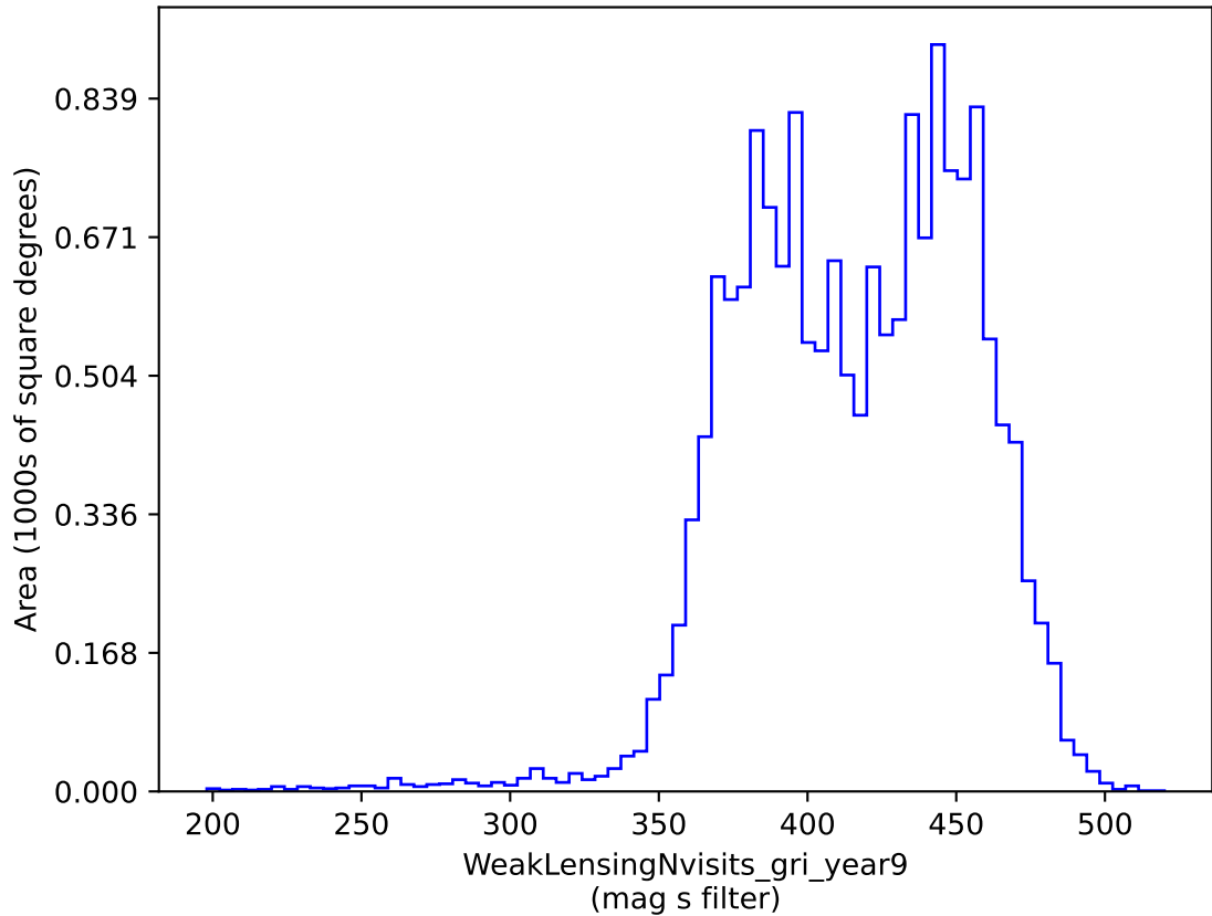
weather_cloudso18v3.4_10yrs gri band non-DD: WeakLensingNvisits_gri_year9
