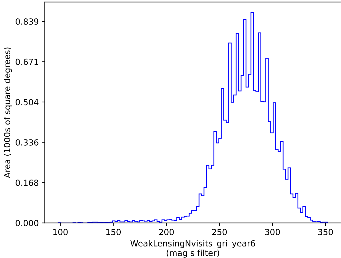
weather_cloudso18v3.4_10yrs gri band non-DD: WeakLensingNvisits_gri_year6
