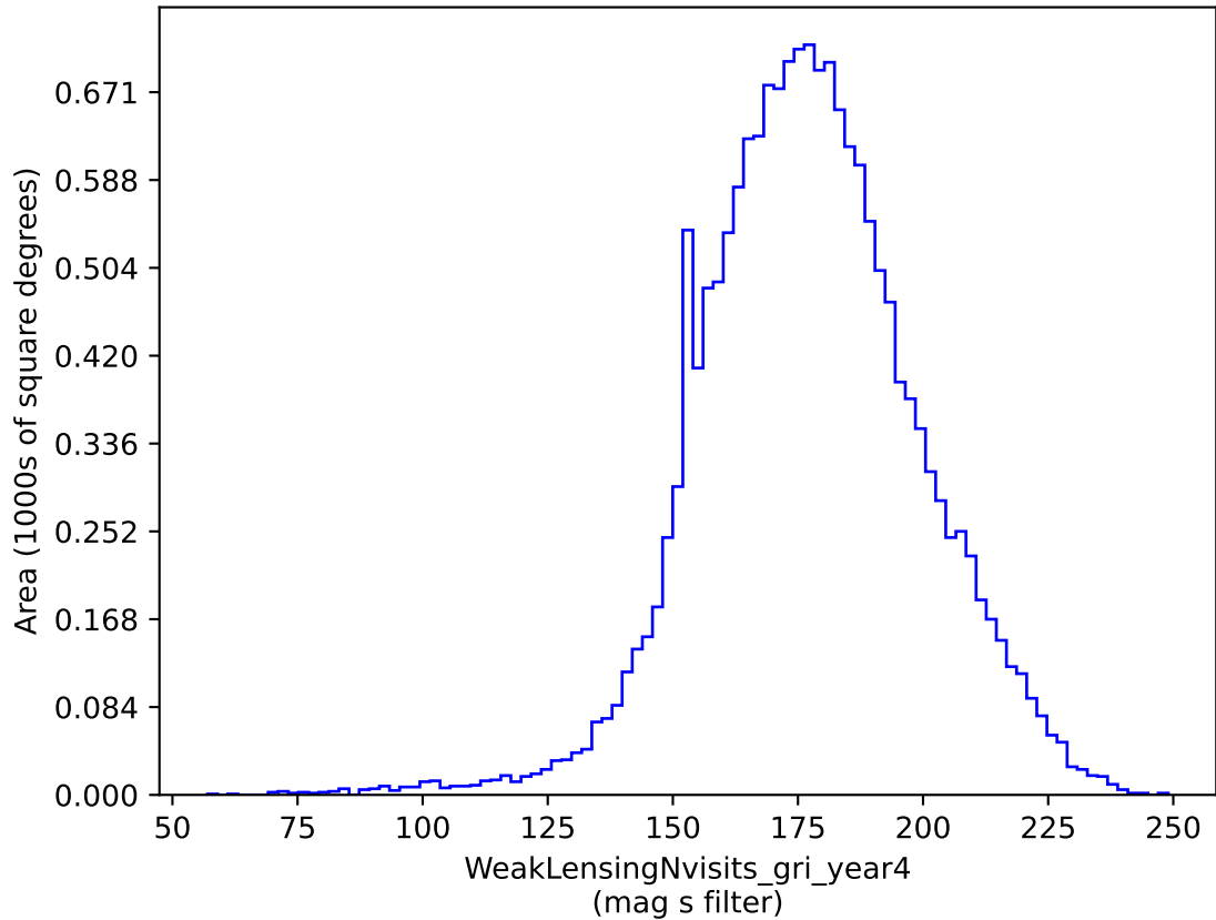
weather_cloudso18v3.4_10yrs gri band non-DD: WeakLensingNvisits_gri_year4
