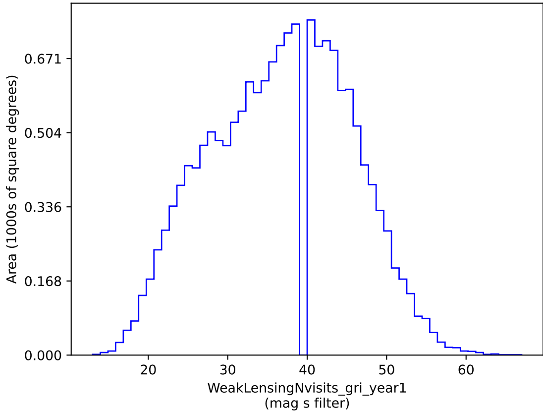
weather_cloudso18v3.4_10yrs gri band non-DD: WeakLensingNvisits_gri_year1
